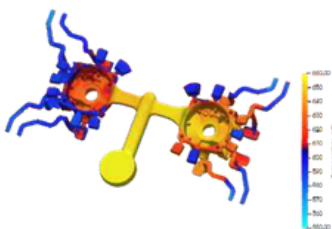
METAL FLOW ANALYSIS
